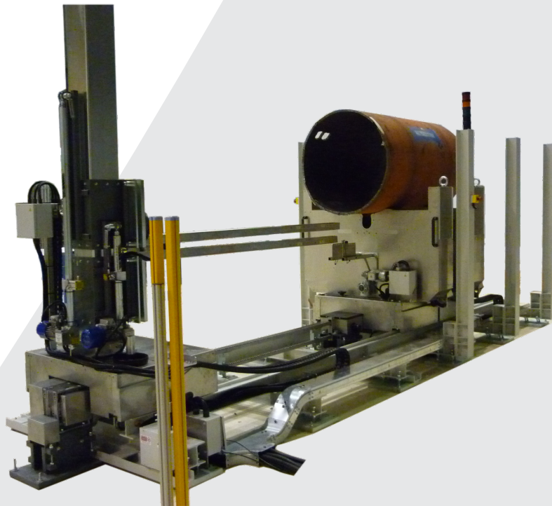
PIPE SCANNER with large pipe lodged on the supports
